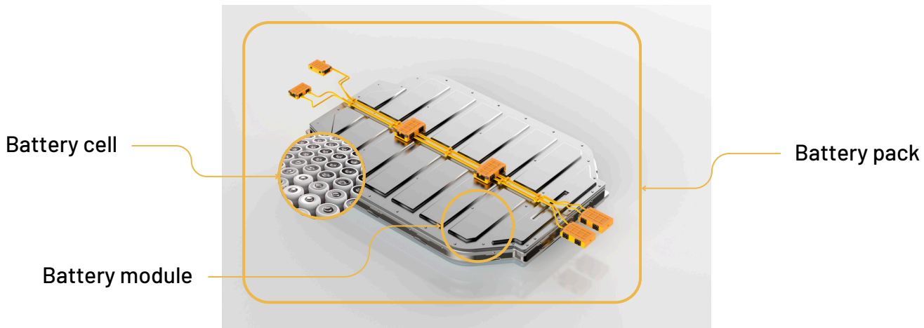
FIGURE 1: EV battery cell, module, pack
